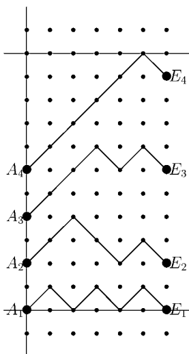
Fig. 1. A star of p = 4 vicious walkers, of length m = 6 , confined to a strip of width h = 11 .
